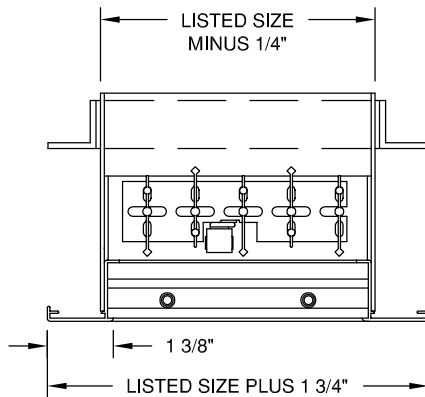
MODEL - SGLFD - 15 - O - WITH SLEEVE AND COLLAR
