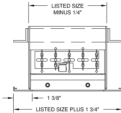
MODEL - SG LFD - WITH SLEEVE, COLLAR AND OPTIONAL OBD
